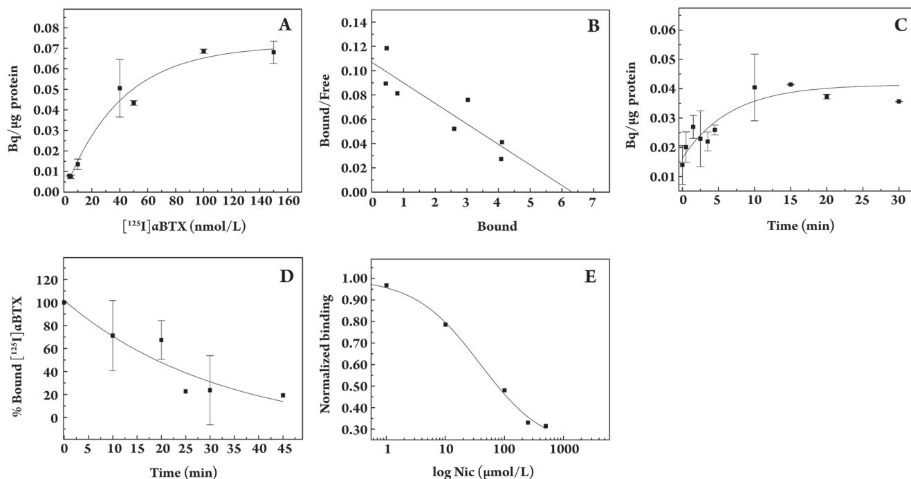
Figure 3. Equilibrium binding of [^{125}\text{I}]\alpha\text{BTX} to SHE-P1-h \alpha 7 -Ric-3 cells. A) Cells were incubated with [^{125}\text{I}]\alpha\text{BTX} for 15 min at the indicated concentrations. B) Scatchard plot corresponding to the data shown in (A). B_{\text{max}} , the maximum number of binding sites, was estimated to be 233.19 fmol/mg protein and the K_D=54.92 nmol/L. (C) Radiolabeled toxin association kinetics. Cells were incubated for the indicated times with 40 nmol/L [^{125}\text{I}]\alpha\text{BTX} . Half-time was reached at about 7.0 min. (D) Cells were incubated with 40 nmol/L [^{125}\text{I}]\alpha\text{BTX} for 15 min, washed thrice and samples collected for radioactivity measurements at the indicated times, yielding a t_{1/2} about 20 min. Data are mean values \pm SD of at least three different samples. E) Inhibition by nicotine of the initial rate of [^{125}\text{I}]\alpha\text{BTX} binding to SHE-P1-h \alpha 7 -Ric-3 cells. Cells were incubated with the indicated concentrations of nicotine at RT for 10 min. [^{125}\text{I}]\alpha\text{BTX} (40 nmol/L) was then added for an additional 15 min at 4 °C. The calculated \text{IC}_{50} is about 40 \mu\text{mol/L} .
